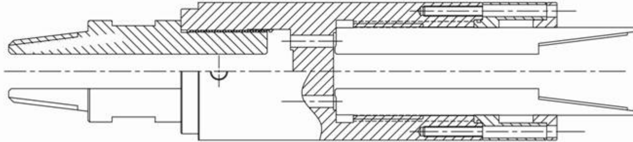
Pin Up x Box Down type (under Rotary Head)
